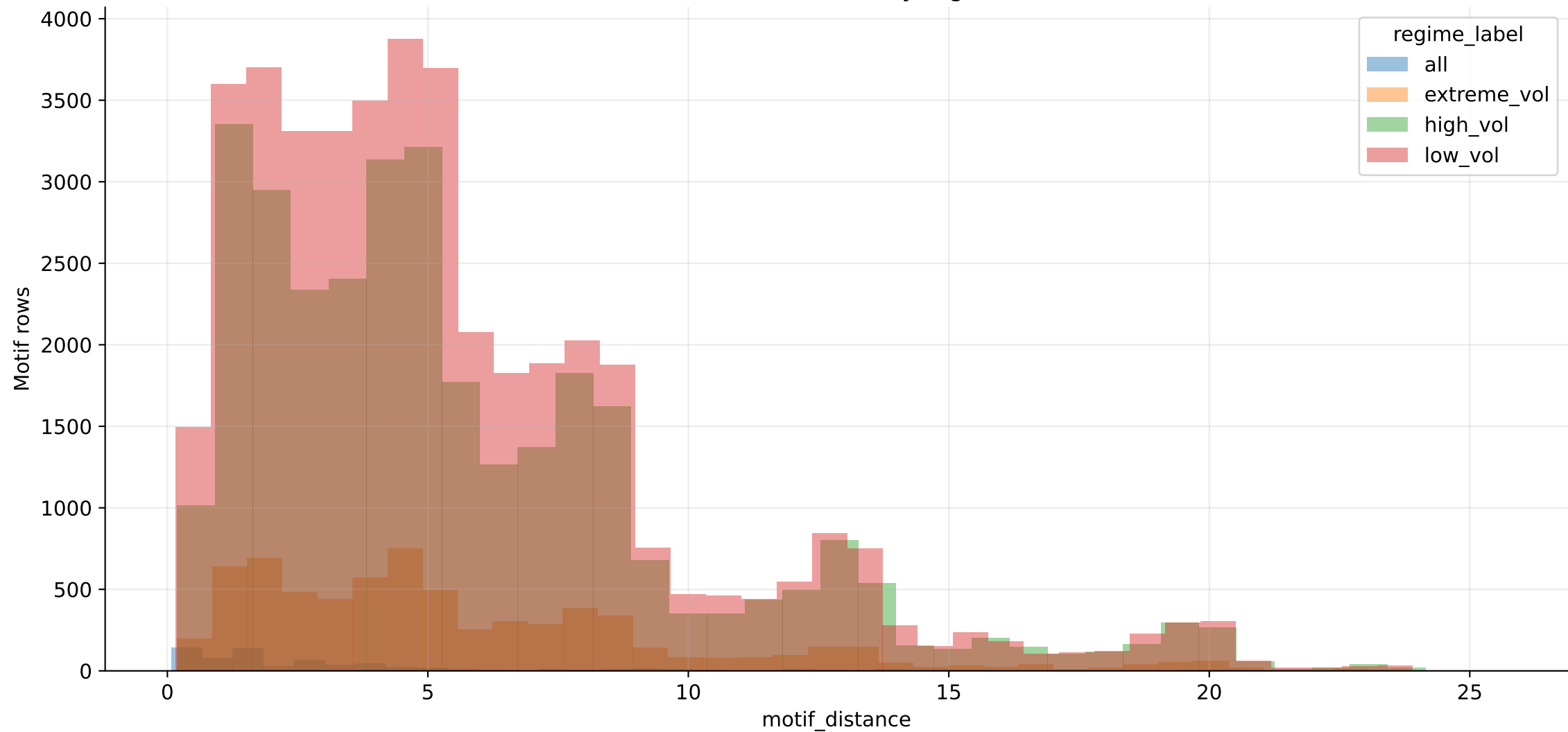
Matrix Profile distances by regime label
